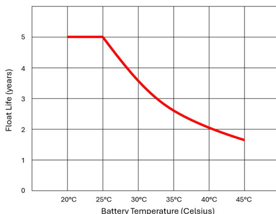
Float Service Life @ 25°C
